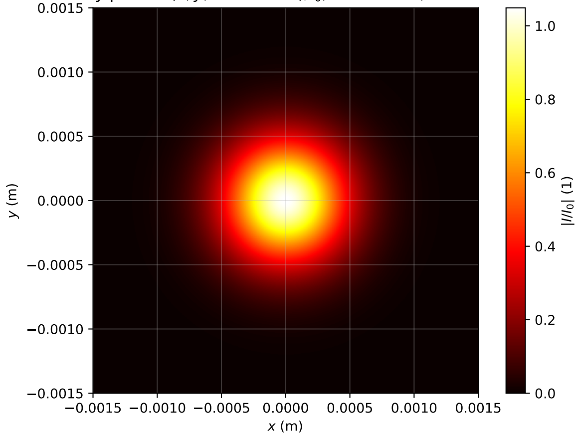
Intensity profile I(x, y, z = 0.557m)/I_0 , Pin=0.5Pcr, artificial time
